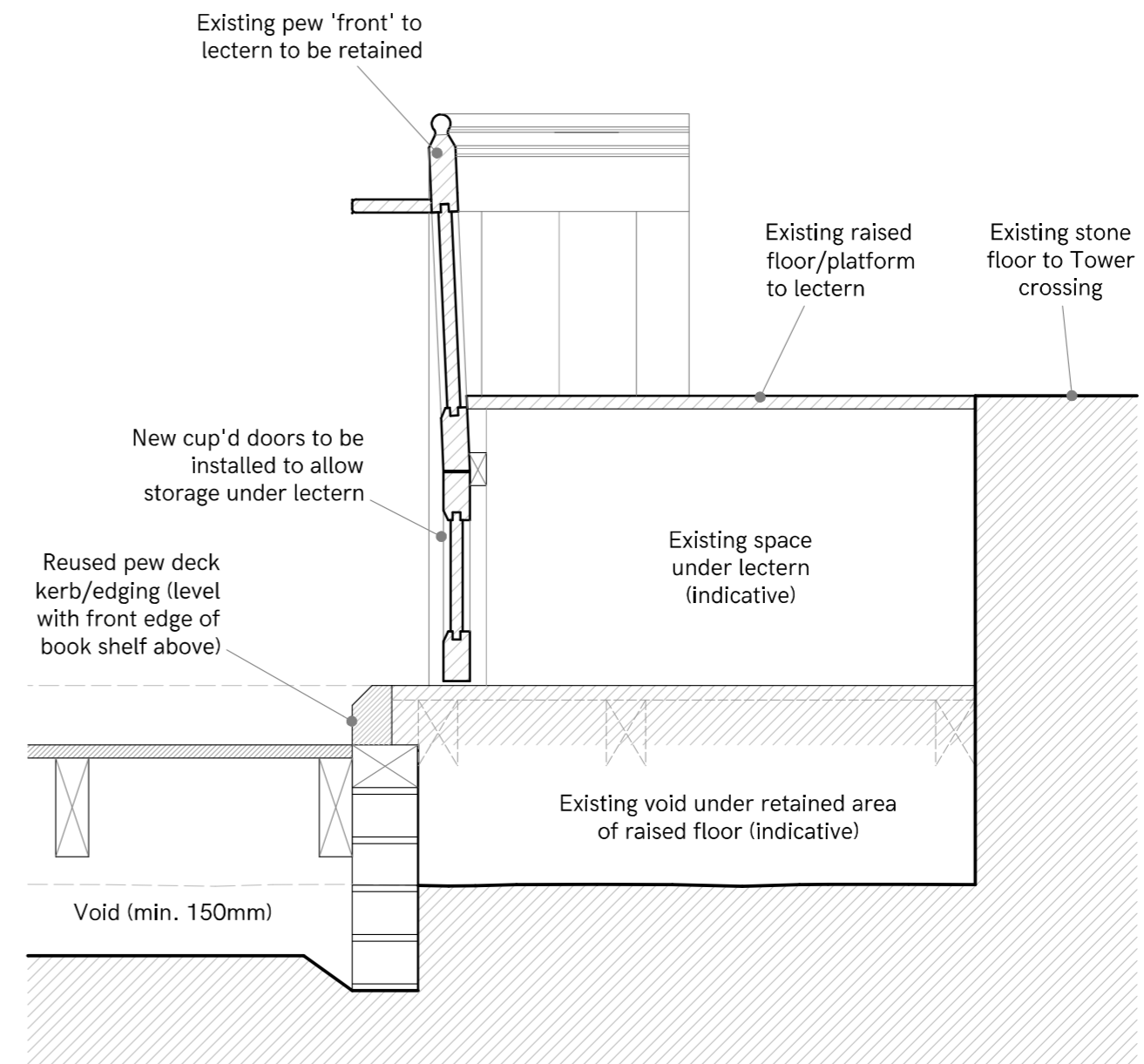
SECTION G-G
